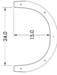
BYOS 2 Flume Dimensions
