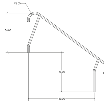
Deck Mounted Stair Rail (MER-1004)
