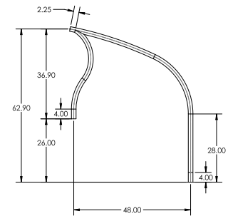
DR-D2S Deck to Stair Handrail
