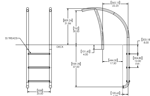
Ladder (ART-1003)
