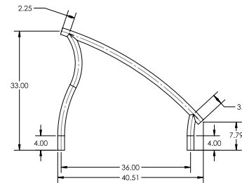
DR-D2D3 Deck to Deck Stair Handrail (pair)
