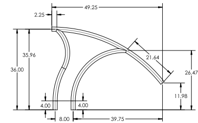
DR-D3D Deck to Deck Return Stair Rail
