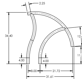
DR-G3D065-S - Single DR-G3D065 - Pair
