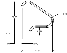
Residential 26-inch Setback
