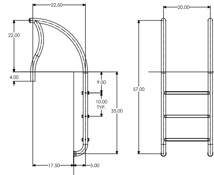
Designer 3 Tread Ladder
