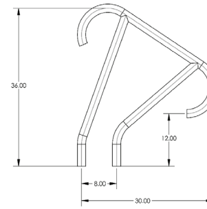
Stair Rail (MER-1002)
