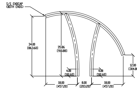
Hand Rail (ART-1001)
