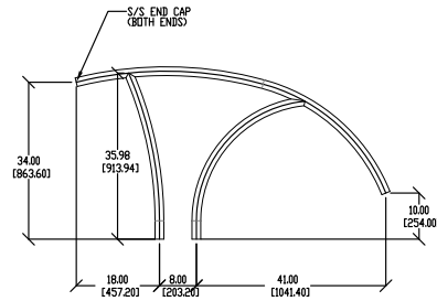
Deck-Mounted Stair Rail (ART-1004)
