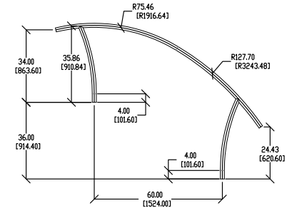
Stair Rail (ART-1002)
