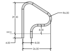
Residential 26-inch Setback
