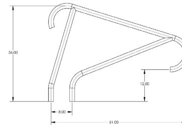
Deck Mounted Stair Rail (MER-1004)
