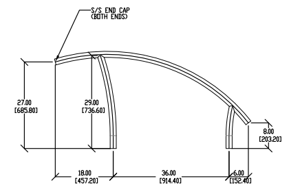
Deck-Mounted Hand Rail (ART-1005)
